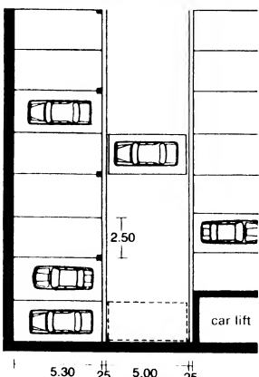
⑪ Plan of garage lift system, ⑫ - ⑬
